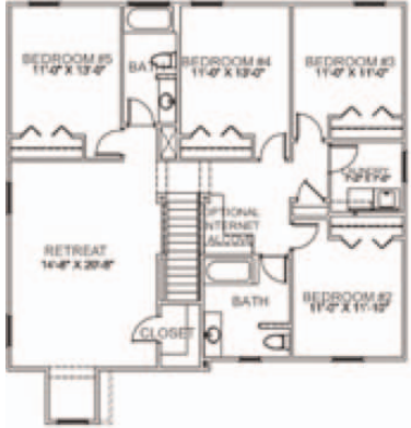
SECOND FLOOR = 5 BEDROOM/ RETREAT
