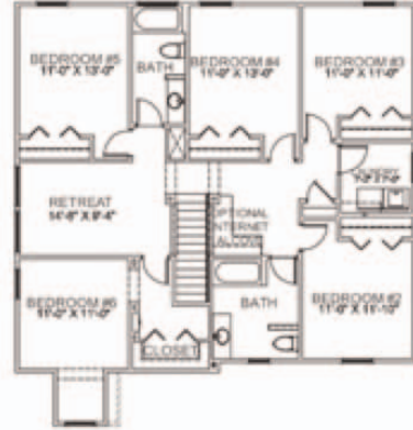
SECOND FLOOR = 6 BEDROOM/ RETREAT
