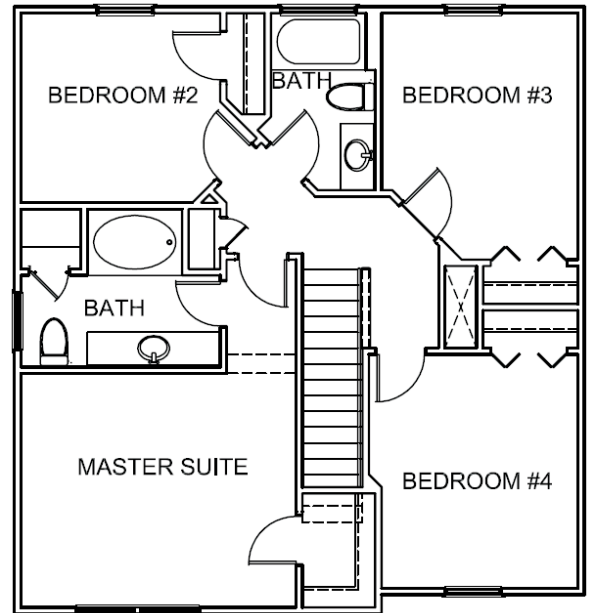
Optional Second Floor 4 Bedroom Plan
